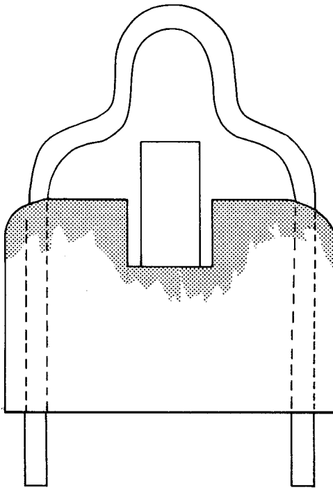
Figure 6-12.—Sight picture 100 yard firing.
