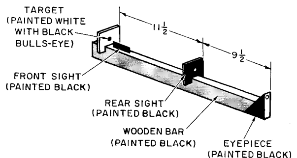
Figure 3-5.—Aiming bar.
