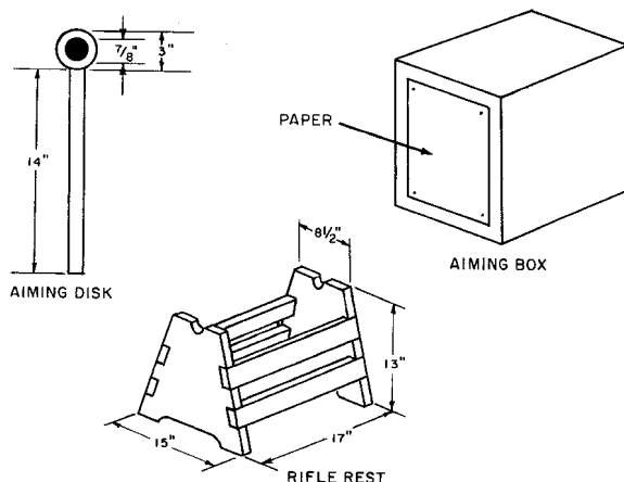
Figure 3-6.—Rifle rest, aiming box and disk.
