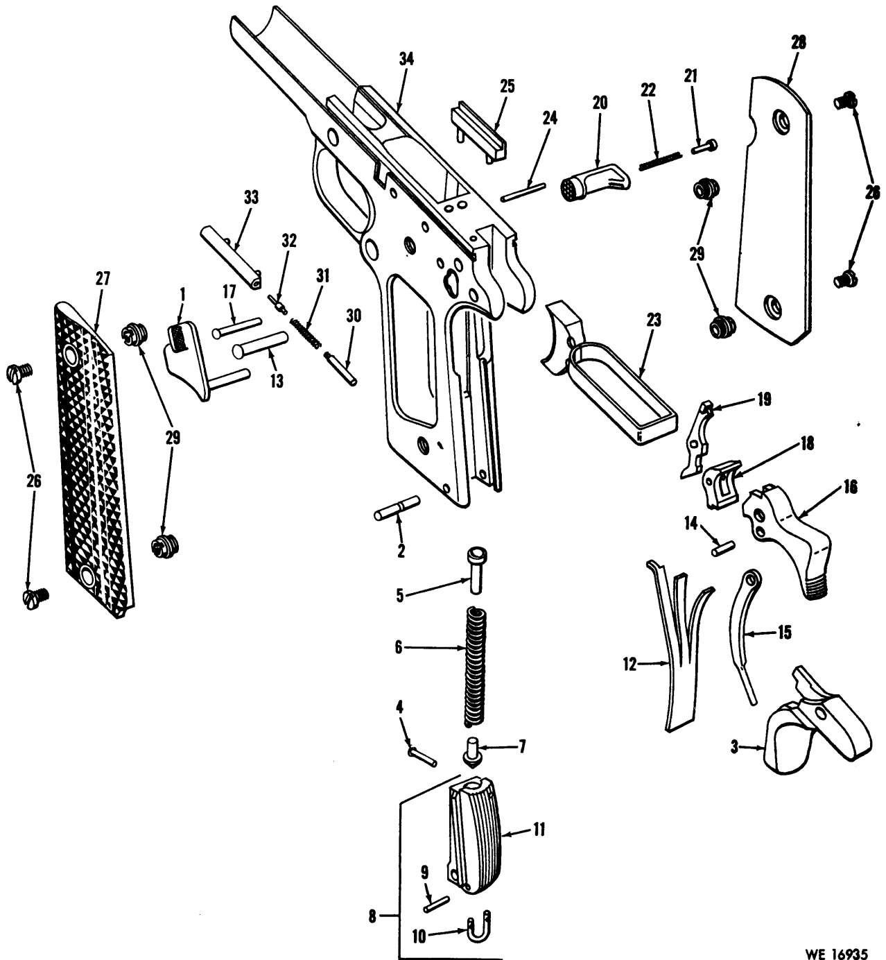
Figurt 5. Receiver group—exploded view
