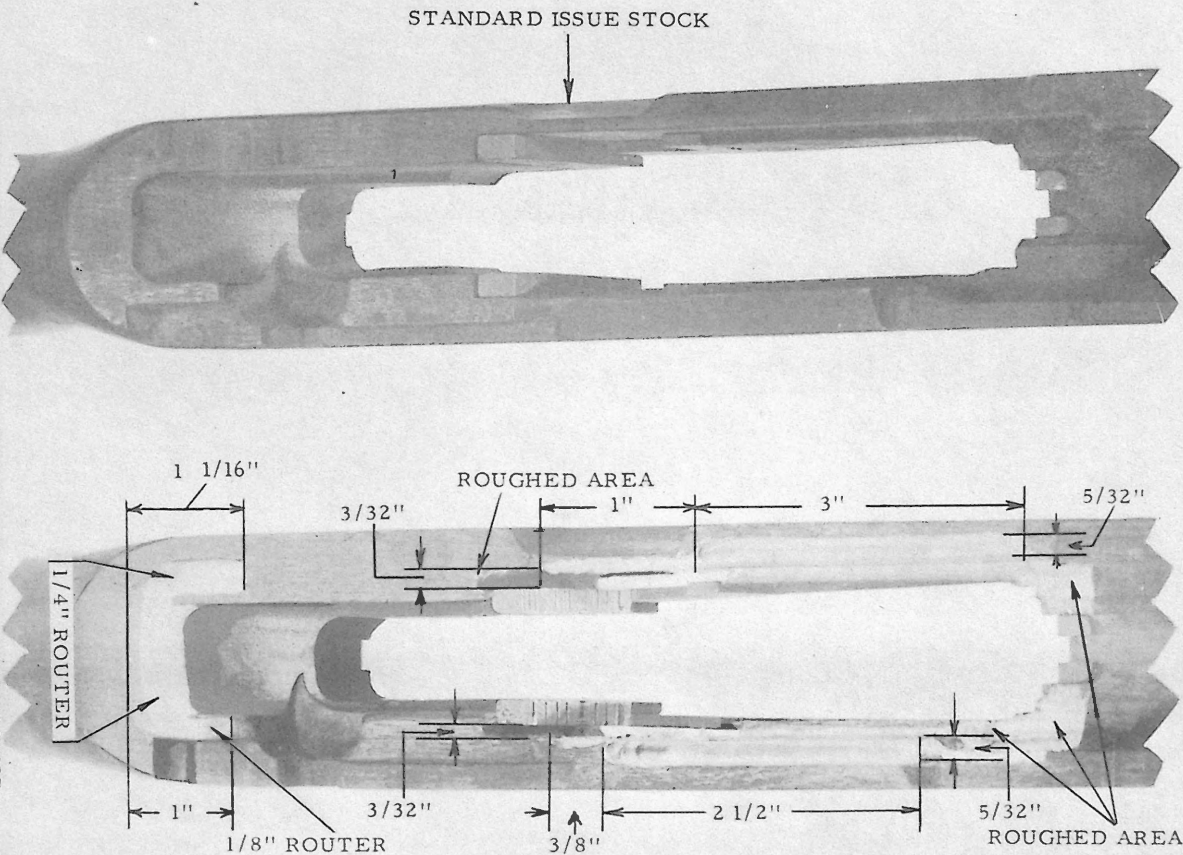
ILLUSTRATION "H 1 " INLETTING FOR GLASS BEDDING
