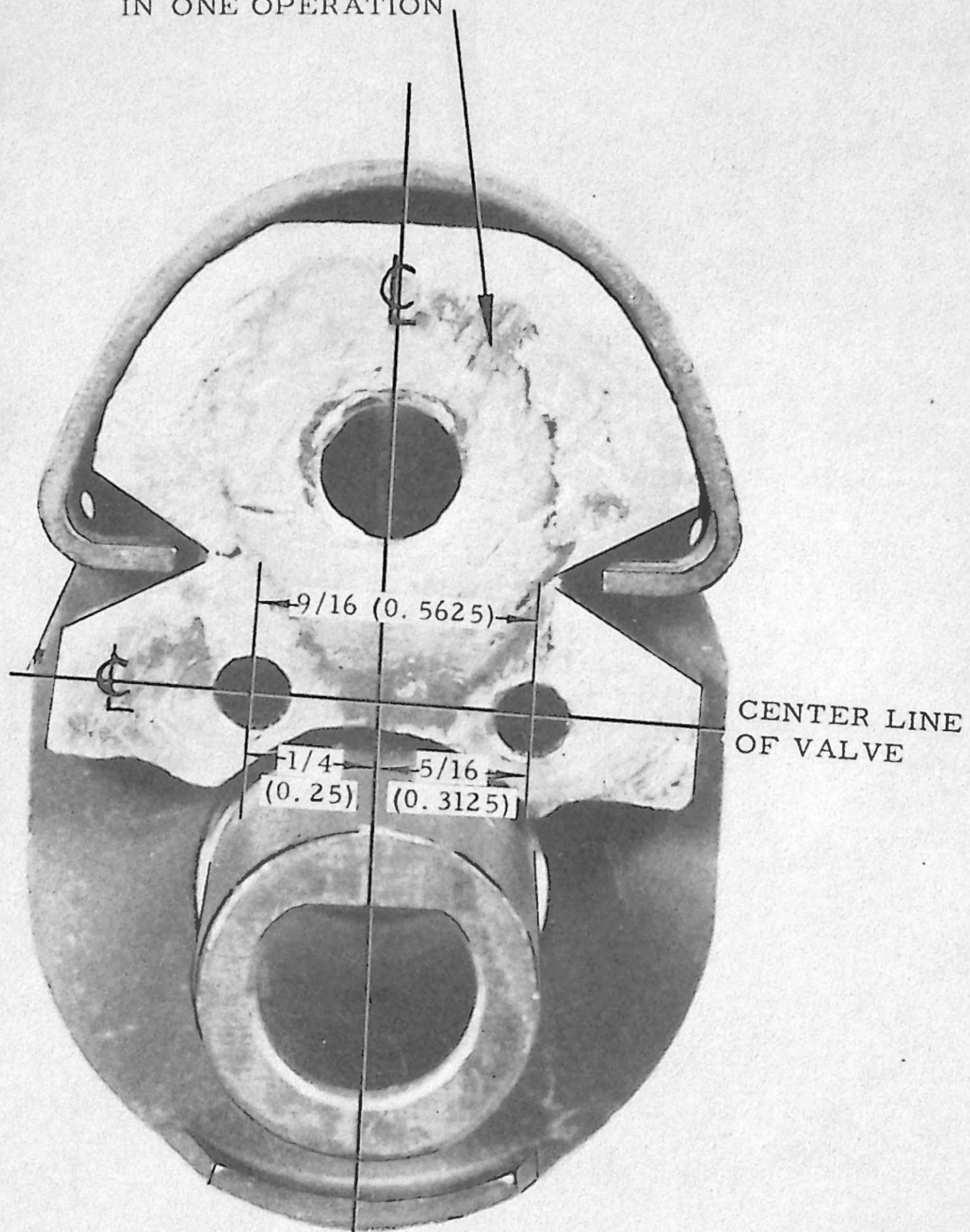
CENTER LINE GAS CYLINDER/BARREL ILLUSTRATION "C" FIXTURE #1
