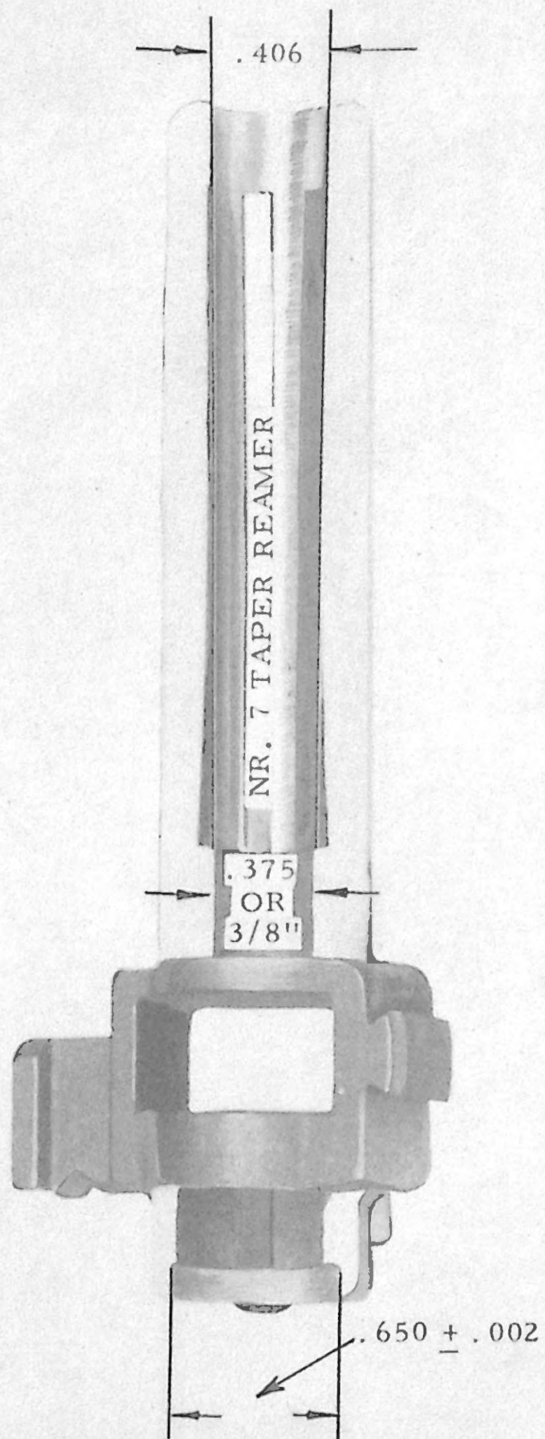
ILLUSTRATION "E 1 " SUPPRESSOR MODIFICATION
